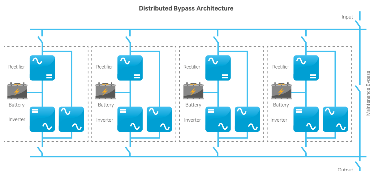
Figure 1: Example of a distributed bypass architecture design.
