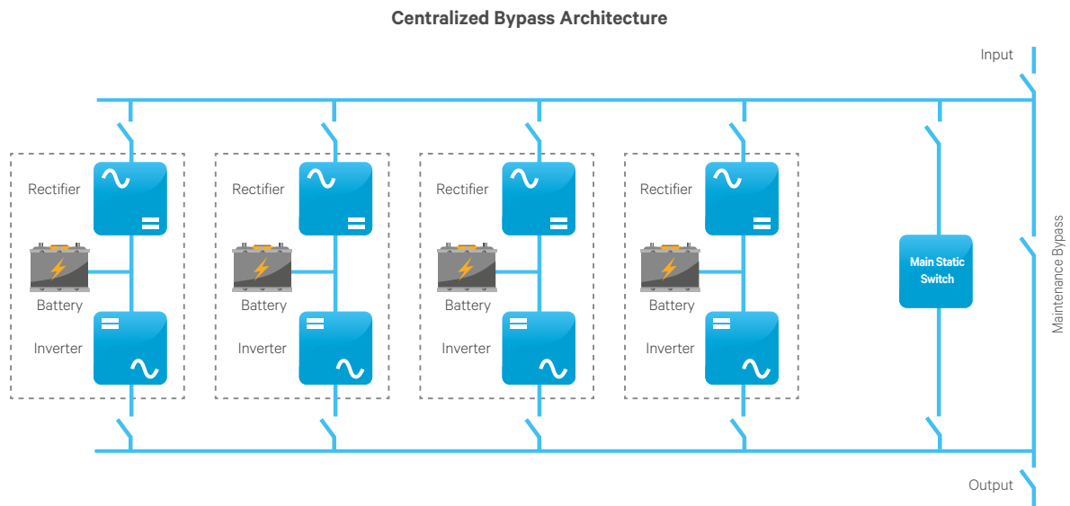
Figure 2: Example of a centralized bypass architecture design.
