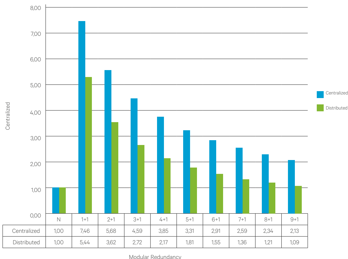
Figure 3: Relative MTBF for centralized and distributed bypass architecture.
